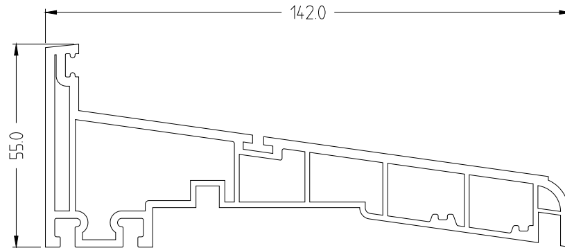
VSW005 CILL ADAPTOR
