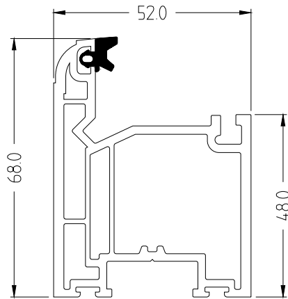
VSW003 MEDIUM BOTTOM SASH
