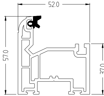
SLIM TOP SASH VSW002
