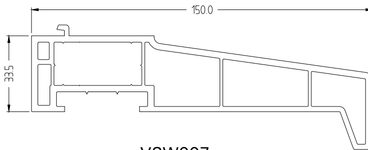
VSW007 150mm CILL
